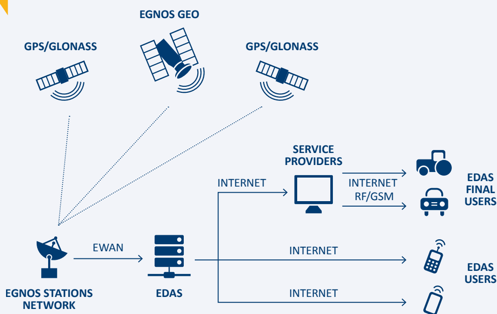
Figure 3.1 EDAS High-Level Architecture
