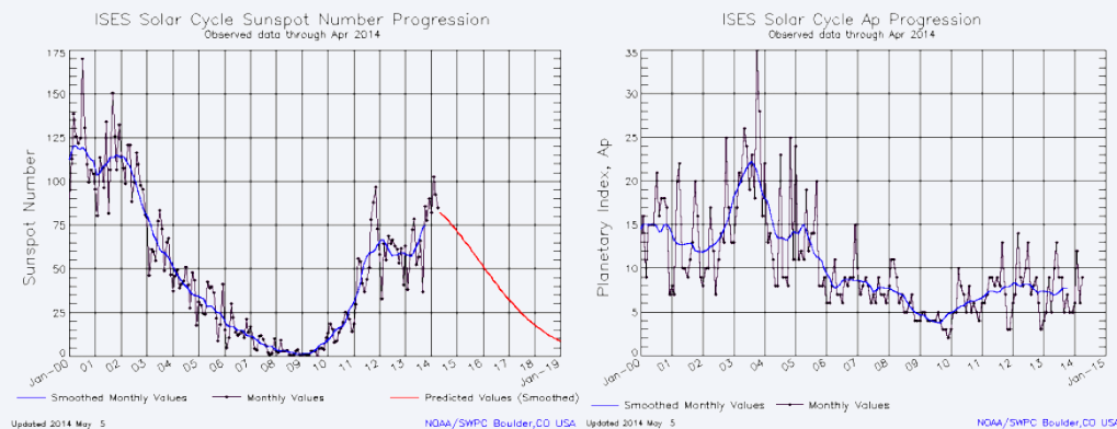
Figure 7.6 SSN (left) and Ap (right) progression from NOAA/SWPC
