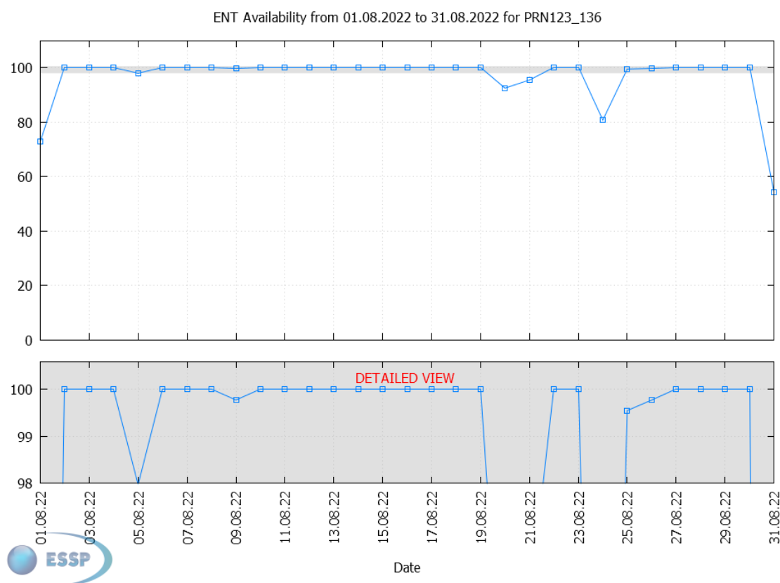
Figure 28 – EGNOS Time Service availability
