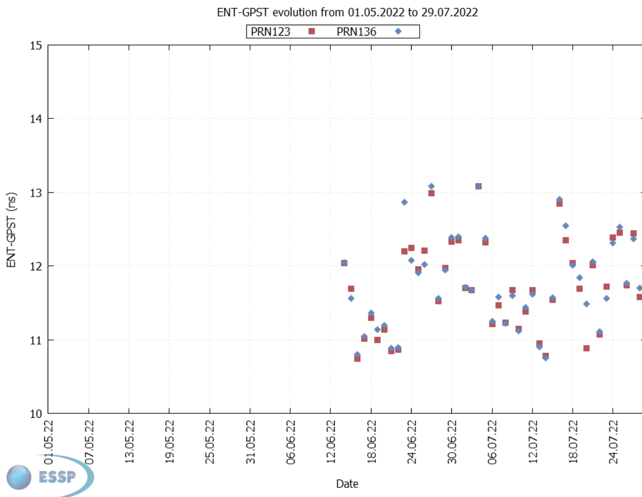
Figure 29 – ENT-GPS offset evolution
