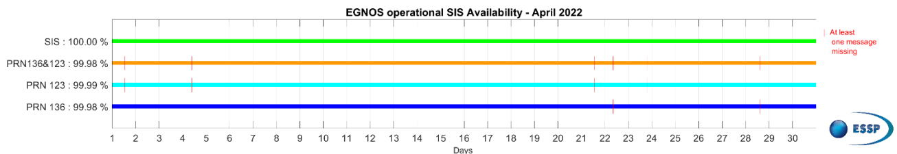
Figure 1 – EGNOS SIS & PRN Availability for April 2022
