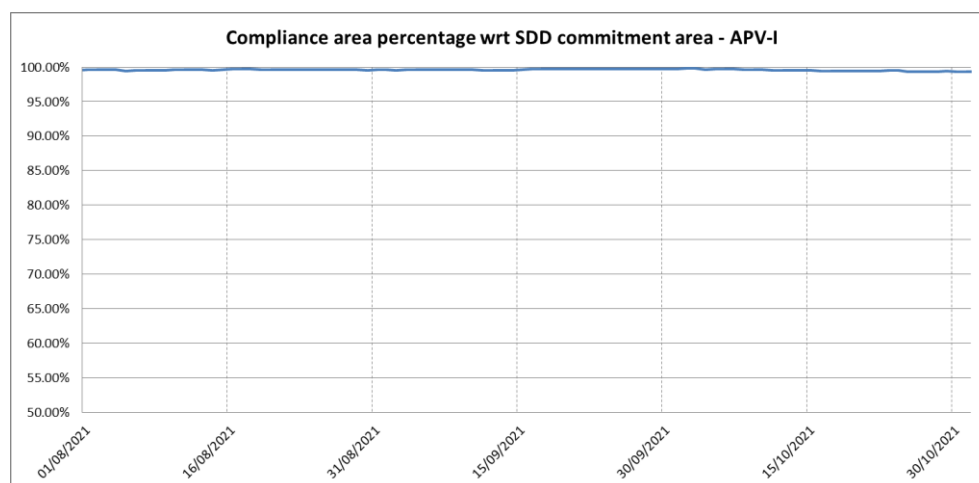
Figure 11 – EGNOS APV-I Availability compliance trend
