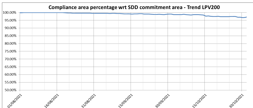
Figure 20 – EGNOS LPV-200 Availability compliance trend
