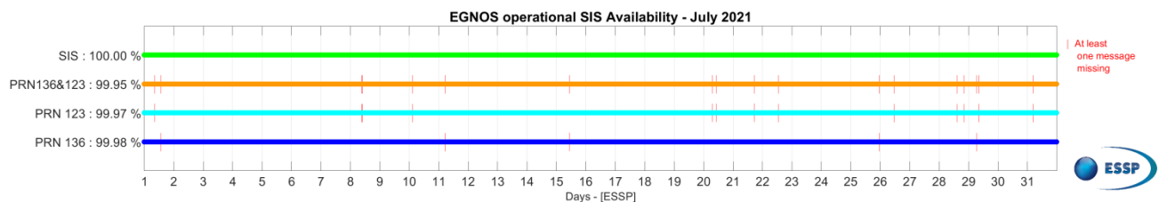
Figure 1 – EGNOS SIS & PRN Availability for July 2021
