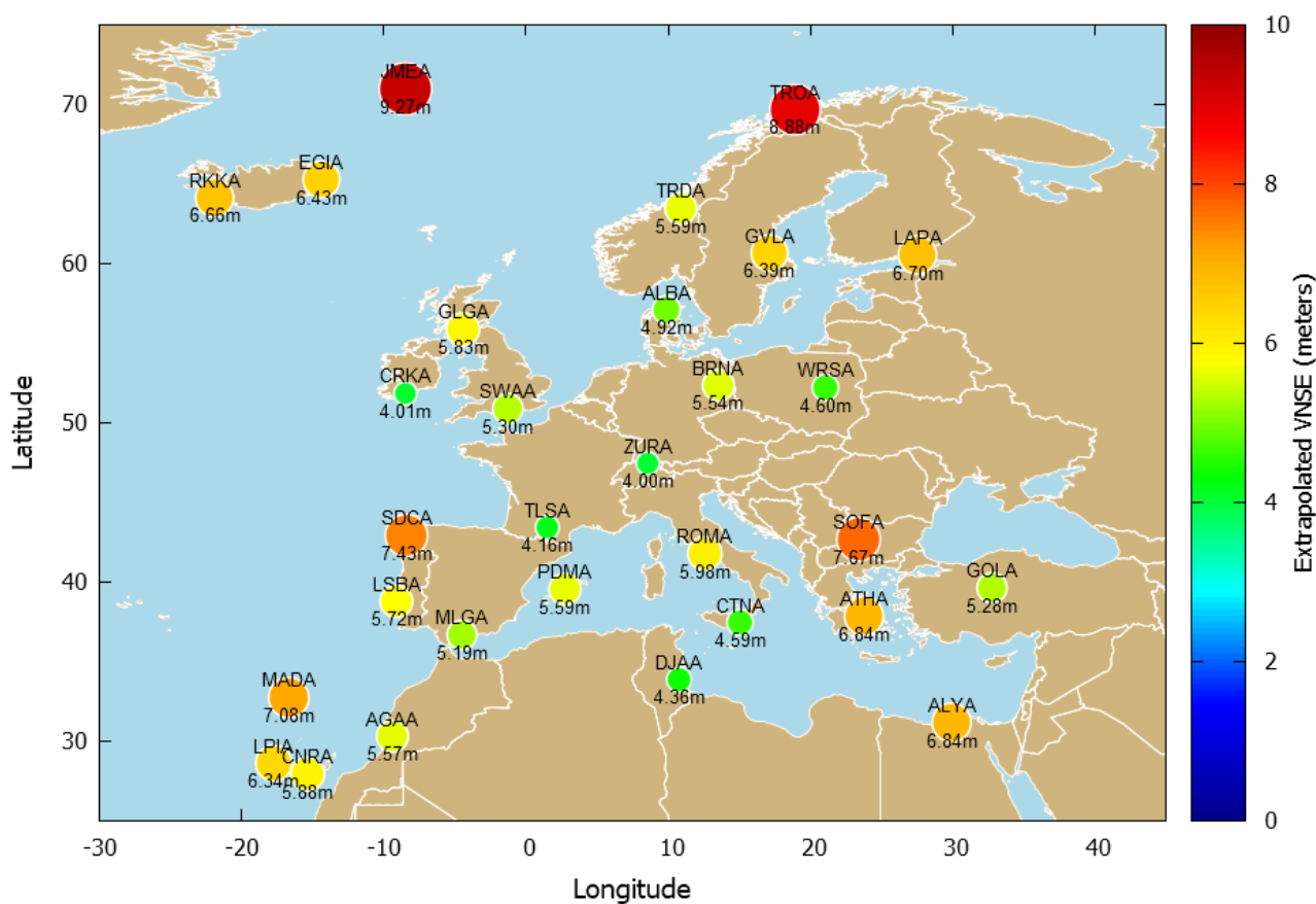
Figure 28 – Extrapolated VNSE at 10^{-7}/150s in the RIMS within the LPV200 commitment
