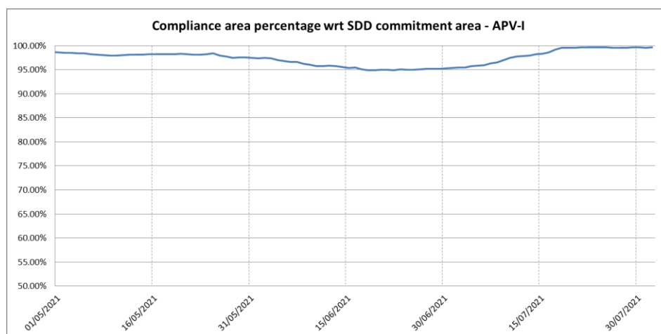
Figure 11 – EGNOS APV-I availability compliance trend
