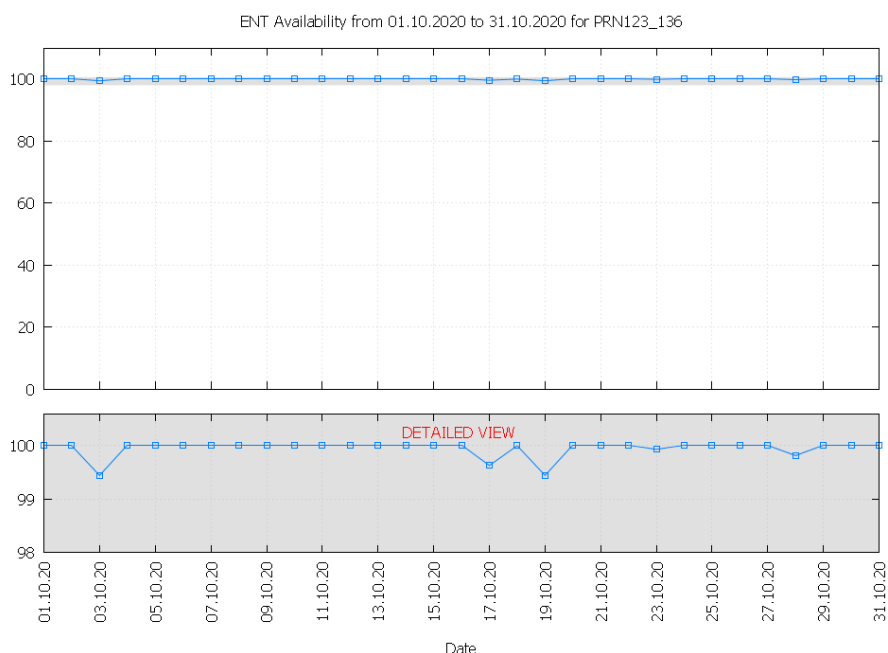
Figure 28 – EGNOS Time Service availability
