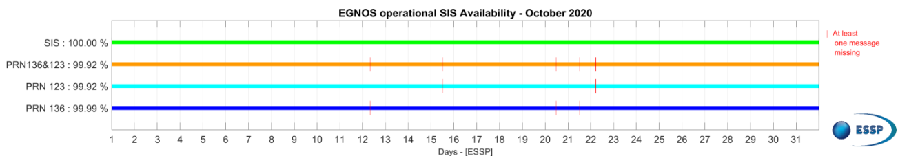
Figure 1 – EGNOS SIS & PRN Availability for October 2020
