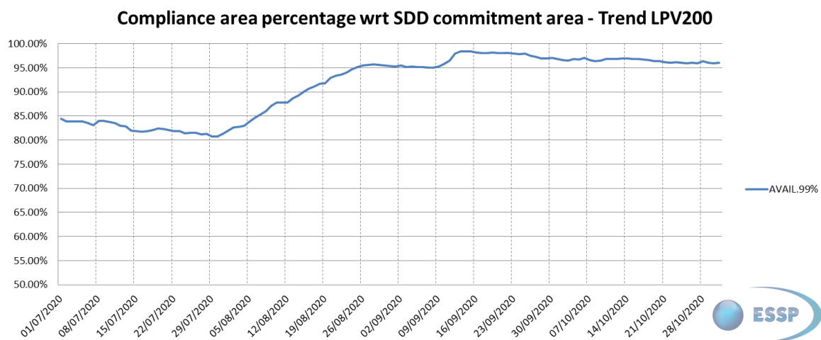
Figure 20 – EGNOS LPV-200 availability compliance trend
