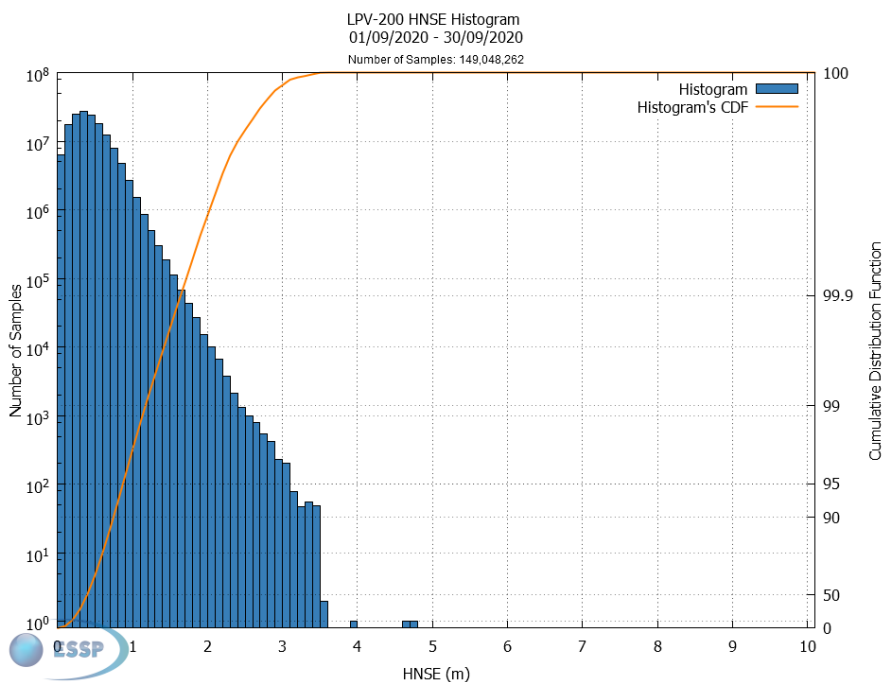
Figure 24 – EGNOS LPV-200 HNSE Histogram and Cumulative Probability
