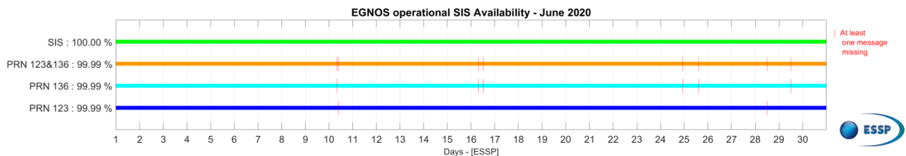
Figure 1 – EGNOS SIS & PRN Availability for June 2020
