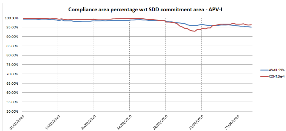
Figure 11 – EGNOS APV-I availability compliance trend
