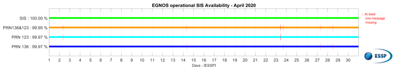
Figure 1 – EGNOS SIS & PRN Availability for April 2020
