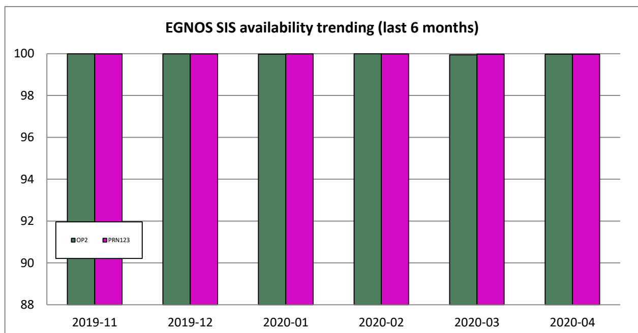
Figure 2 – Trend of EGNOS SIS Availability per GEO 2
