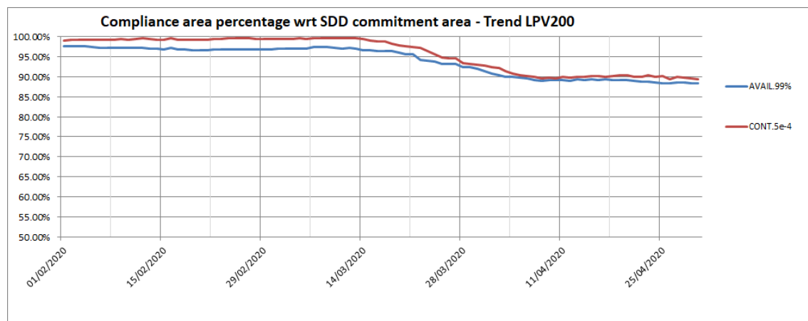
Figure 20 – EGNOS LPV-200 availability compliance trend
