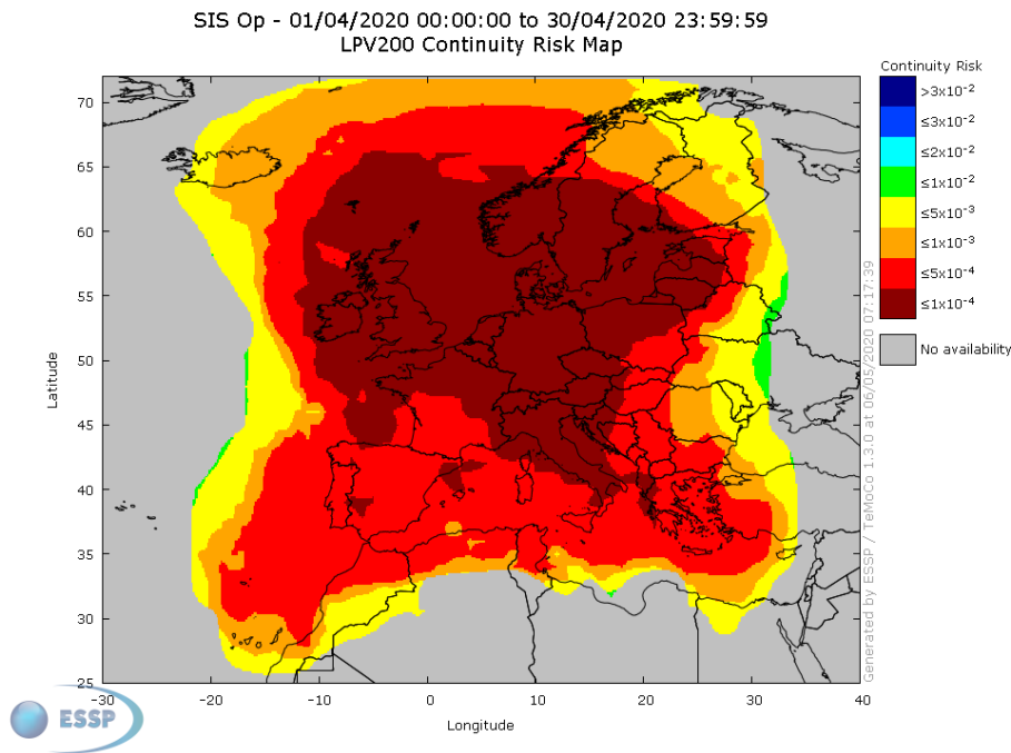
Figure 21 – EGNOS LPV-200 Continuity 4
