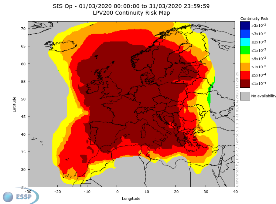
Figure 21 – EGNOS LPV-200 Continuity 4
