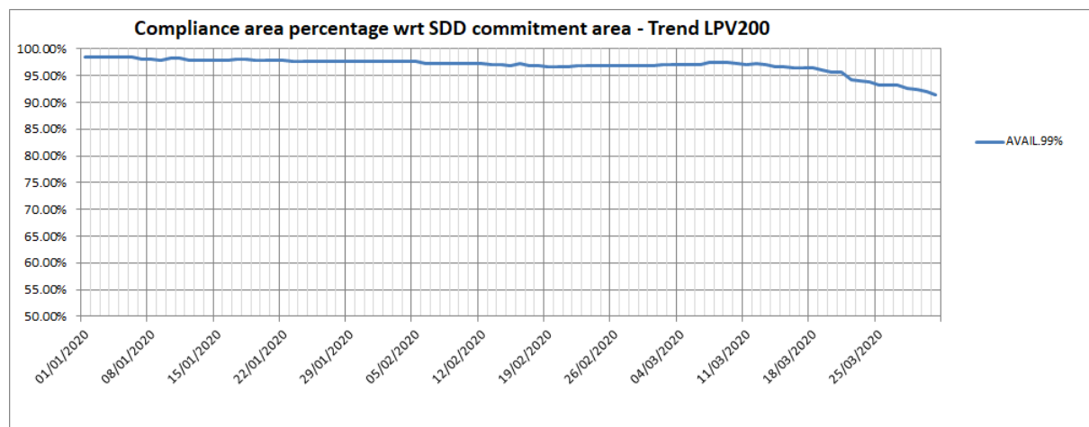
Figure 20 – EGNOS LPV-200 availability compliance trend
