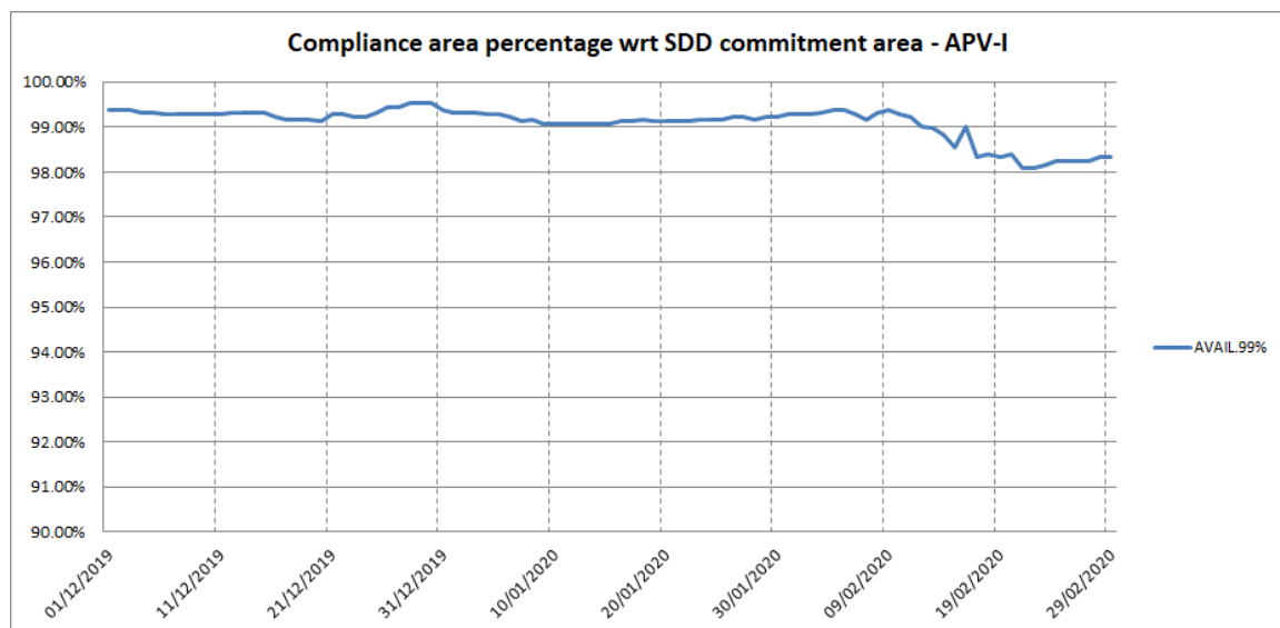
Figure 11 – EGNOS APV-I availability compliance trend
