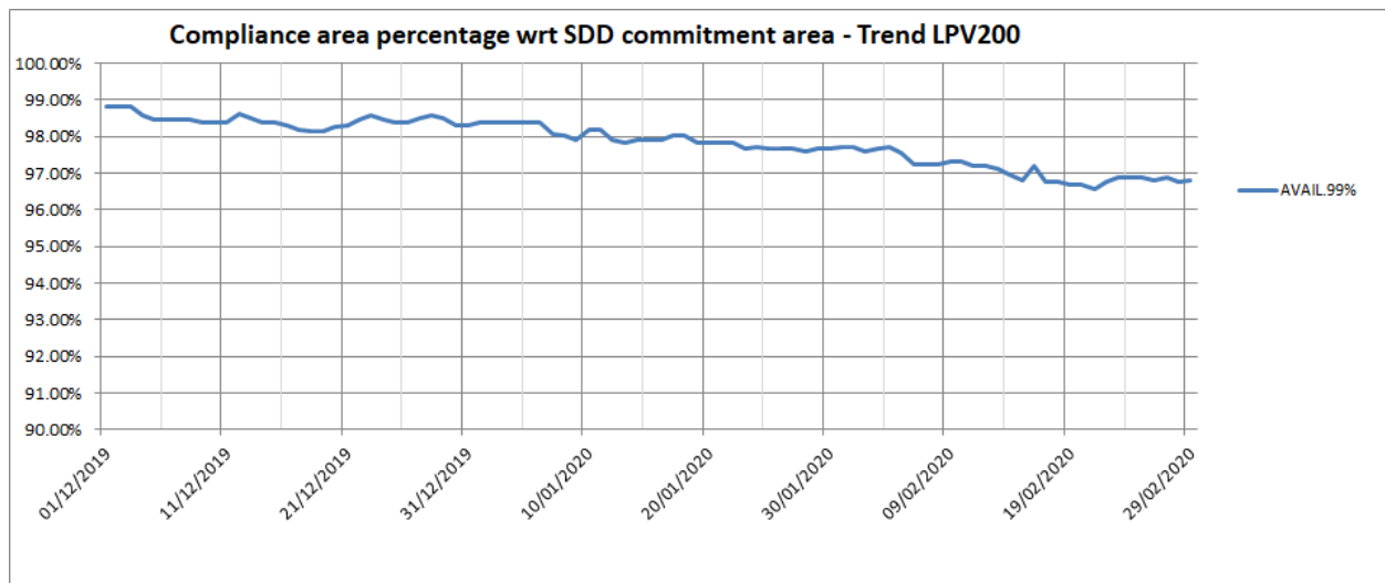
Figure 20 – EGNOS LPV-200 availability compliance trend
