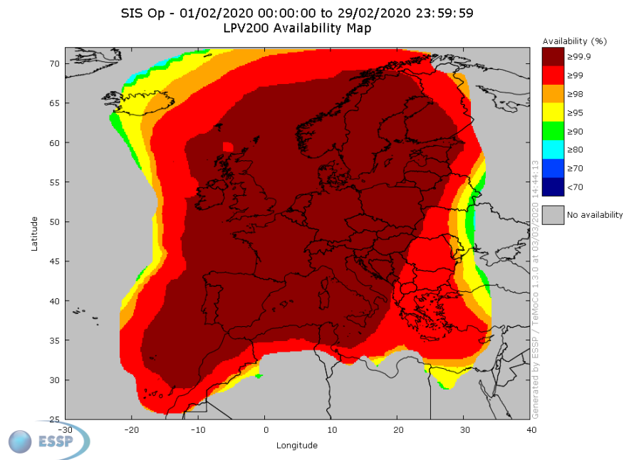
Figure 19 – EGNOS LPV-200 Availability
