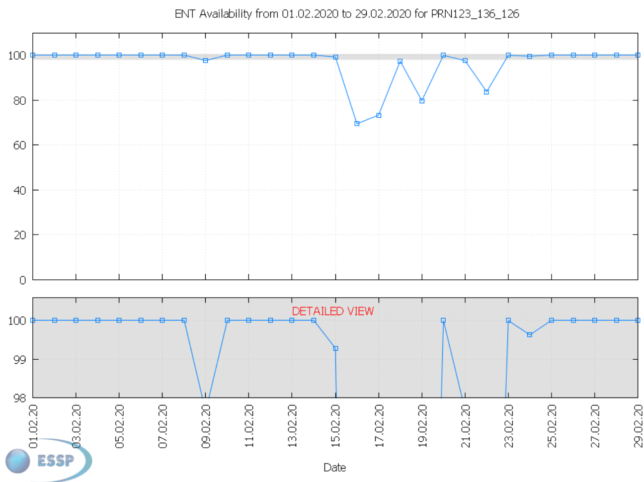
Figure 28 – EGNOS Time Service availability
