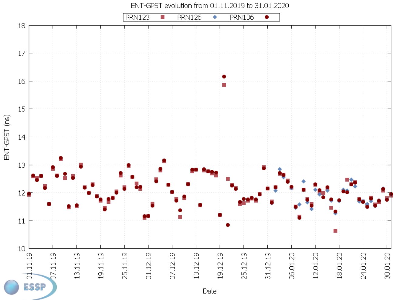
Figure 29 – ENT-GPS offset evolution
