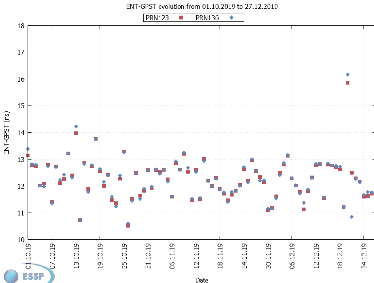
Figure 31 – ENT-GPS offset evolution
