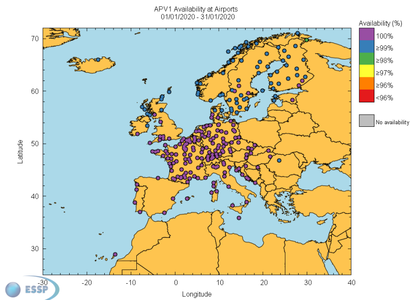
Figure 18 – EGNOS APV-I Availability at airports
