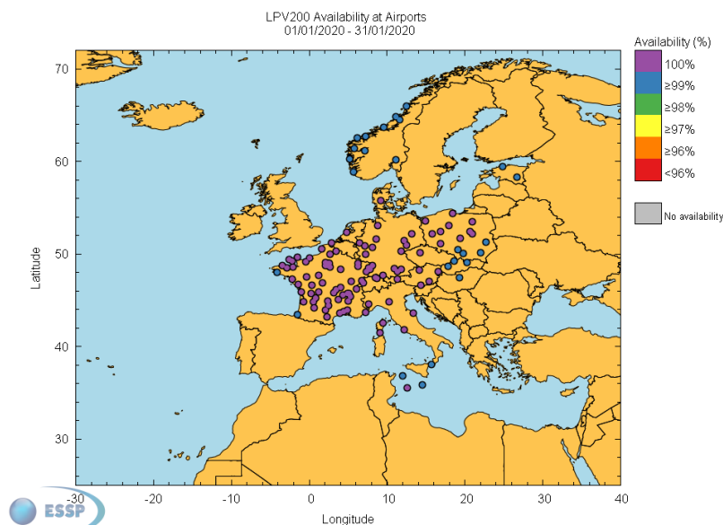
Figure 27 – EGNOS LPV-200 Availability at airports
