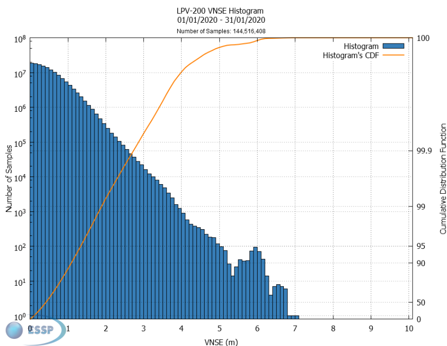
Figure 26 – EGNOS LPV-200 VNSE Histogram and Cumulative Probability
