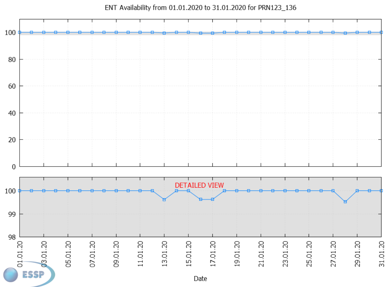
Figure 30 – EGNOS Time Service availability
