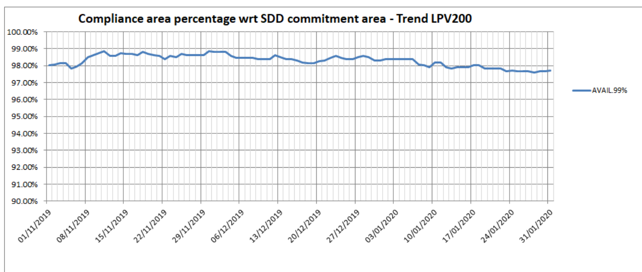
Figure 21 – EGNOS LPV-200 availability compliance trend
