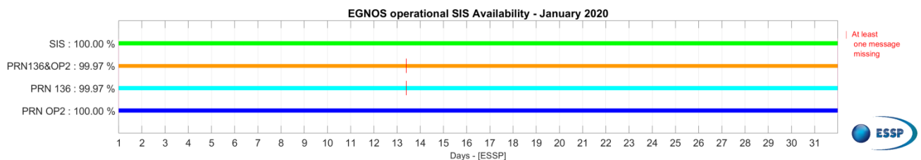
Figure 1 – EGNOS SIS & PRN Availability for January 2020.
