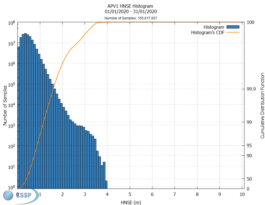
Figure 16 – EGNOS APV-I HNSE Histogram and Cumulative Probability
