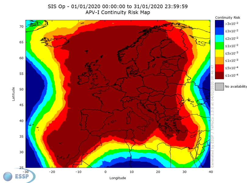
Figure 13 – EGNOS APV-I Continuity
