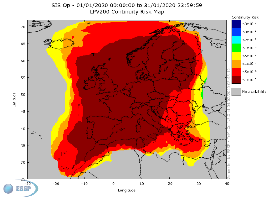
Figure 22 – EGNOS LPV-200 Continuity 3
