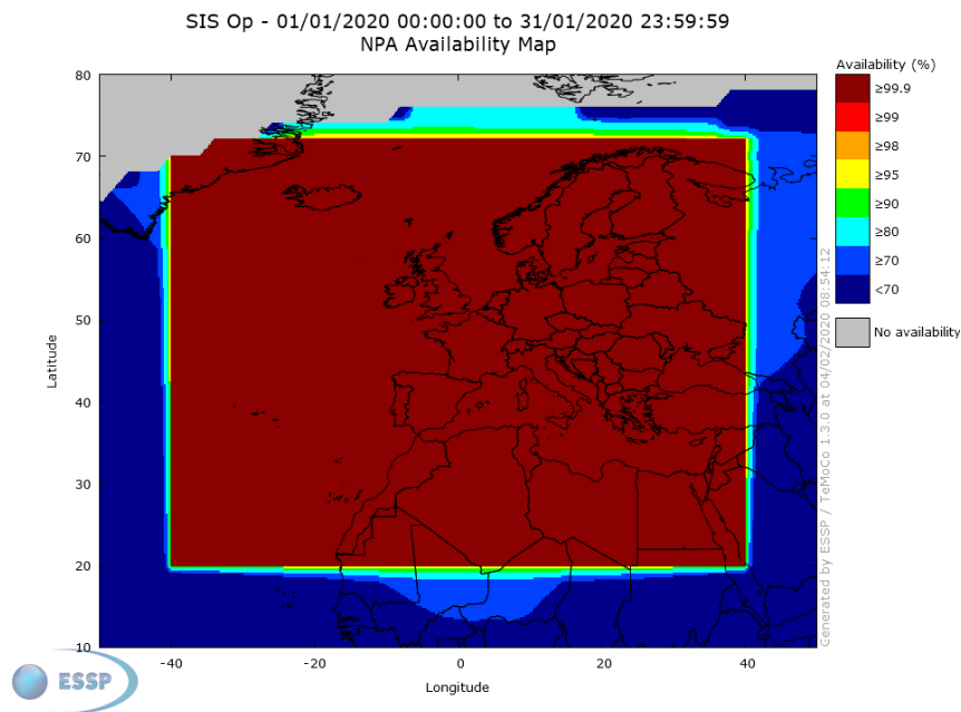
Figure 6 – EGNOS NPA availability
