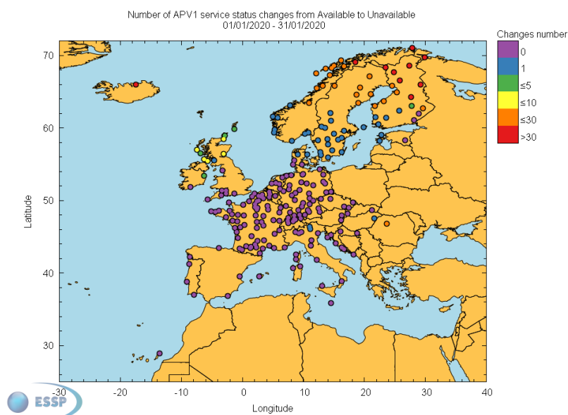
Figure 19 – EGNOS APV-I outages
