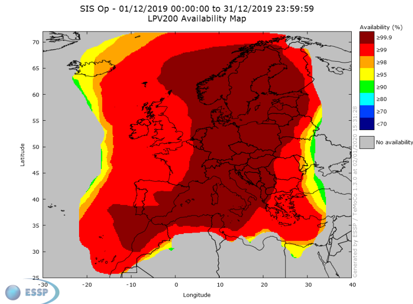
Figure 20 – EGNOS LPV-200 Availability
