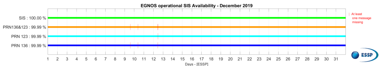
Figure 1 – EGNOS SIS & PRN Availability for December 2019.
