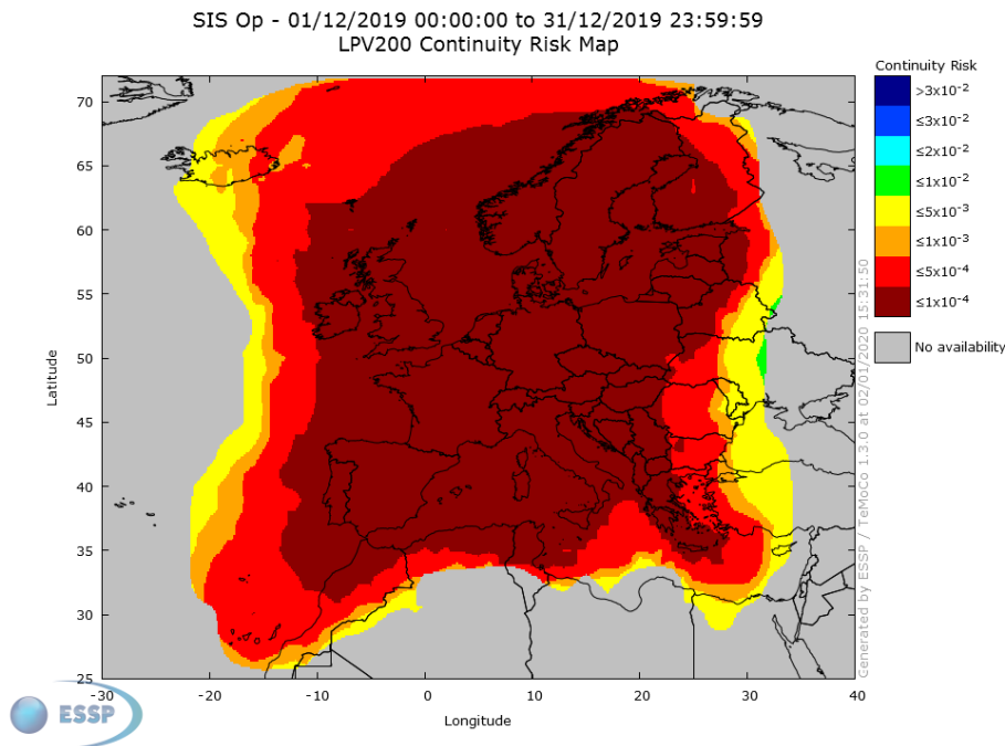
Figure 22 – EGNOS LPV-200 Continuity 2
