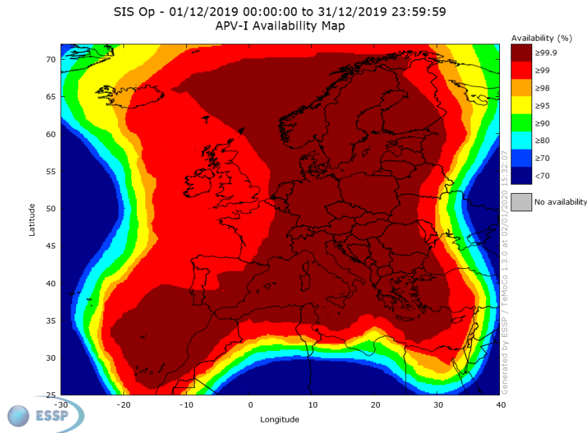
Figure 11 – EGNOS APV-I Availability
