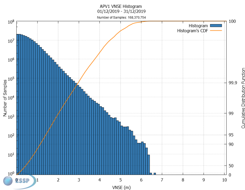
Figure 17 – EGNOS APV-I VNSE Histogram and Cumulative Probability
