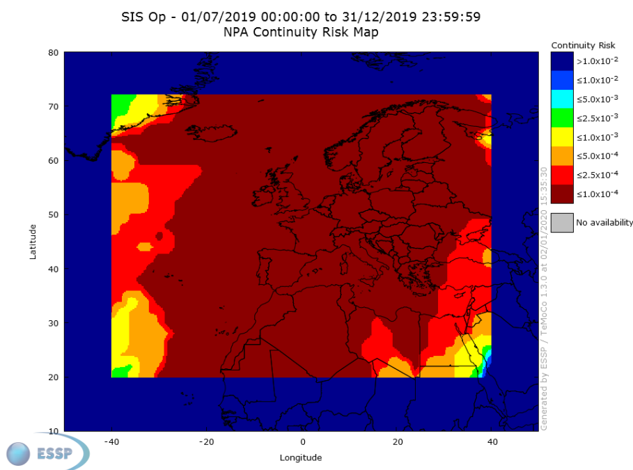
Figure 8 – EGNOS NPA Continuity over the last 6 months
