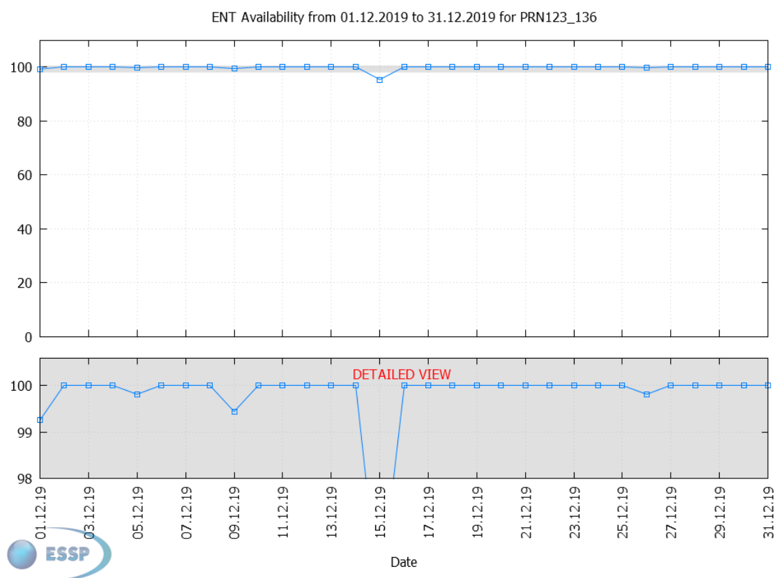
Figure 29 – EGNOS Time Service availability
