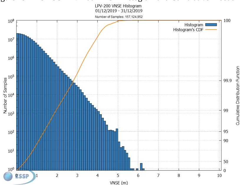
Figure 26 – EGNOS LPV-200 VNSE Histogram and Cumulative Probability
