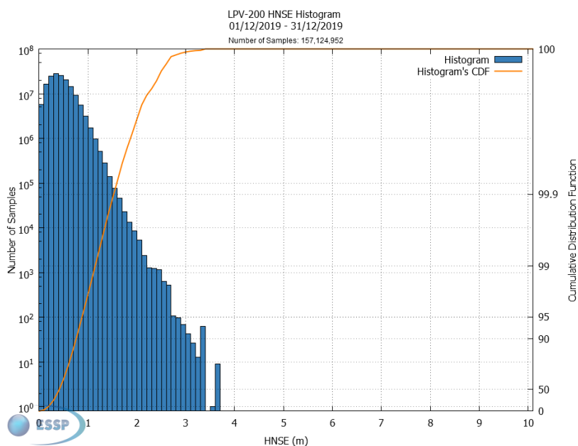
Figure 25 – EGNOS LPV-200 HNSE Histogram and Cumulative Probability
