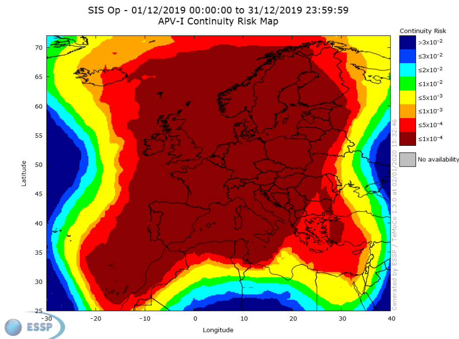
Figure 13 – EGNOS APV-I Continuity
