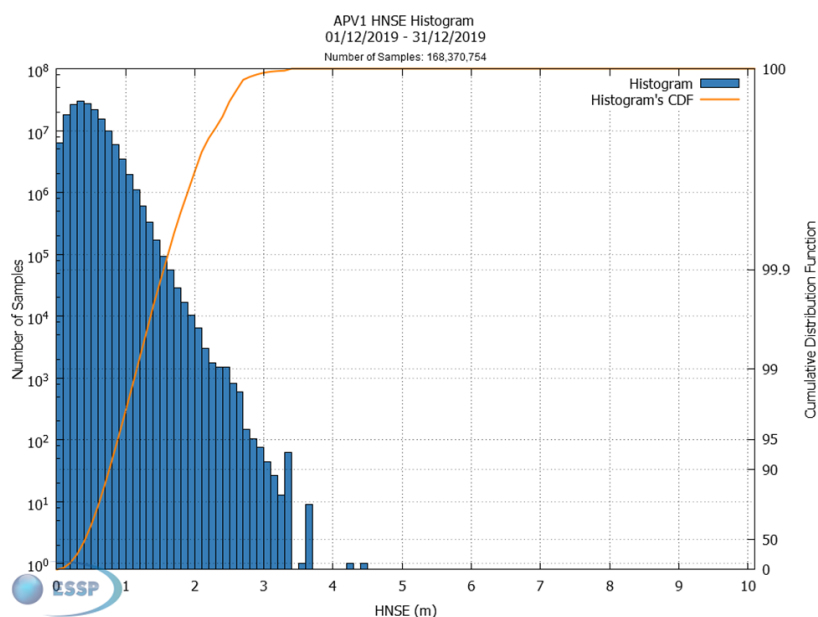
Figure 16 – EGNOS APV-I HNSE Histogram and Cumulative Probability
