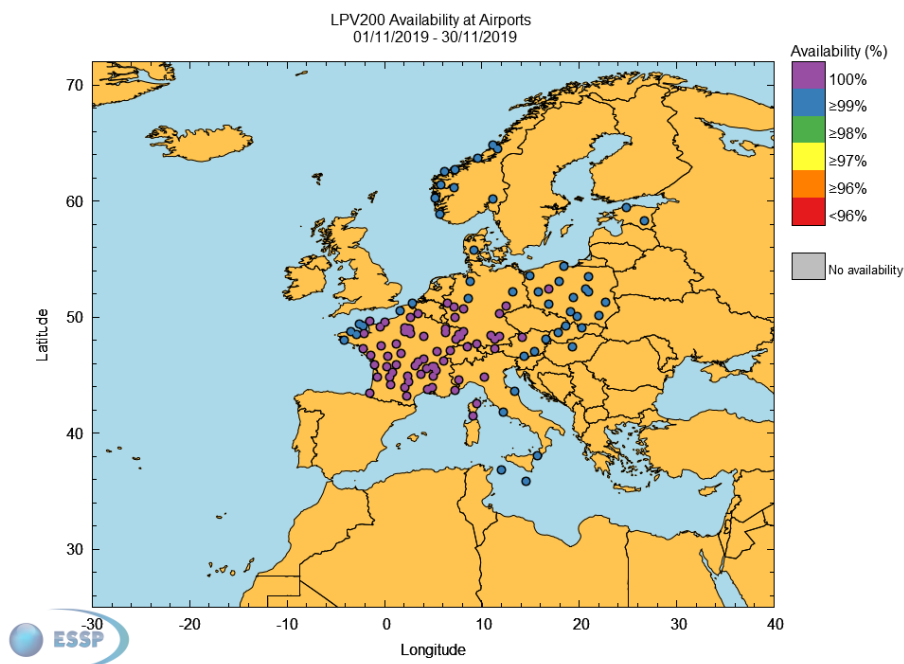
Figure 27 – EGNOS LPV-200 Availability at airports
