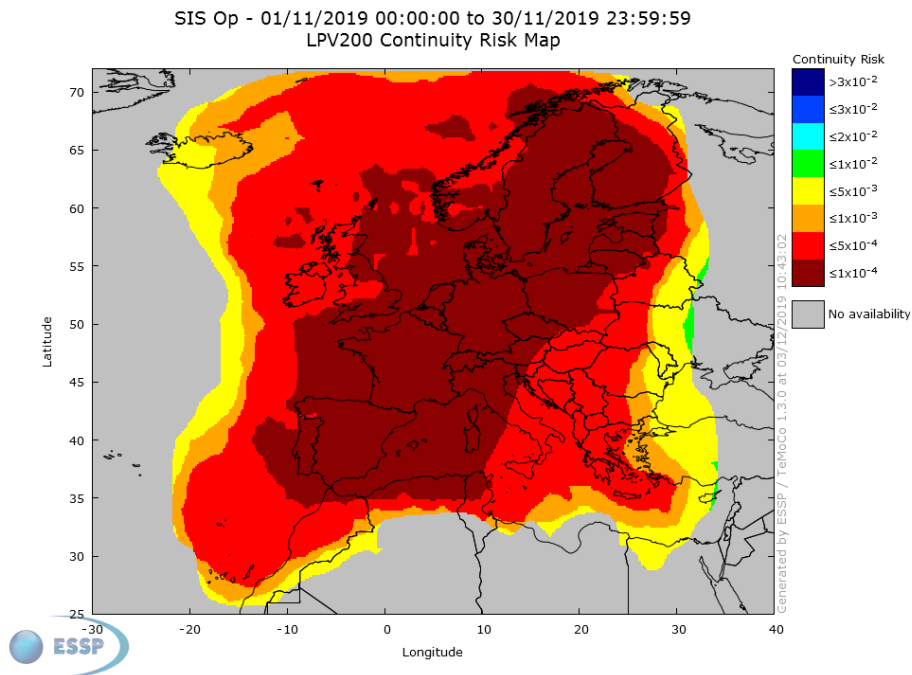
Figure 22 – EGNOS LPV-200 Continuity 2
