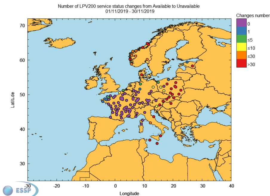
Figure 28 – EGNOS LPV-200 outages
