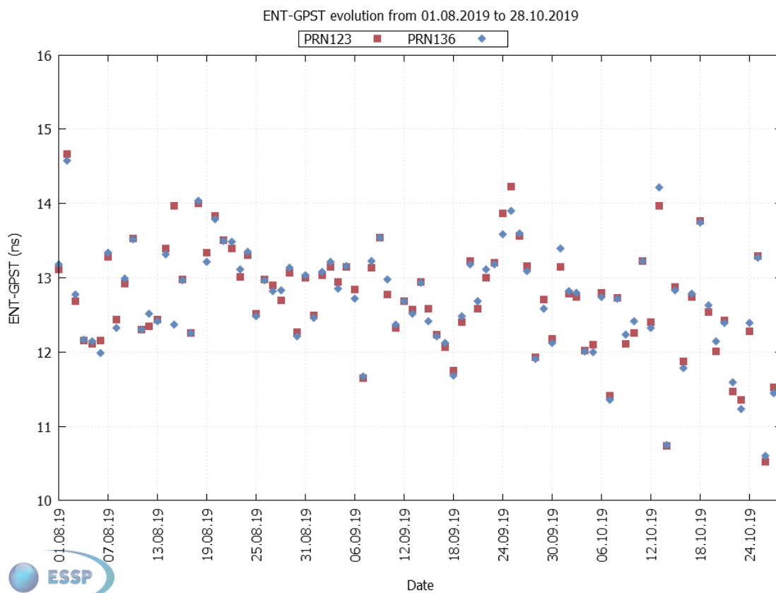
Figure 30 – ENT-GPS offset evolution
