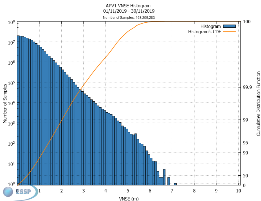
Figure 17 – EGNOS APV-I VNSE Histogram and Cumulative Probability
