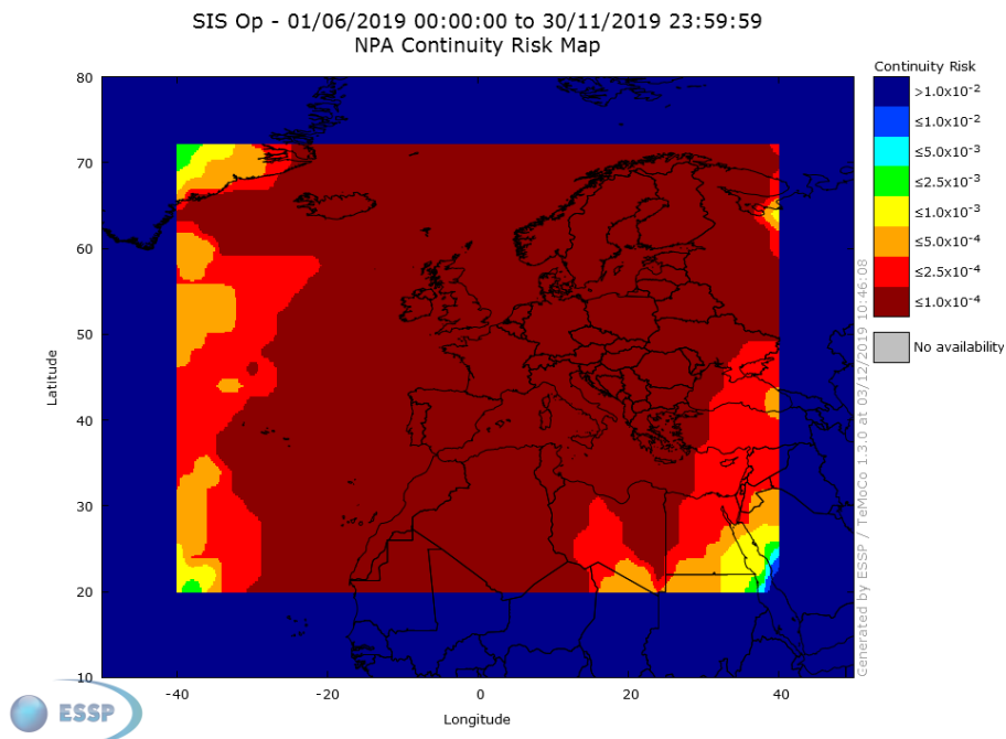
Figure 8 – EGNOS NPA Continuity over the last 6 months
