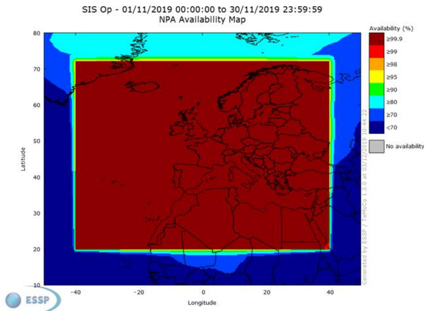
Figure 6 – EGNOS NPA availability
