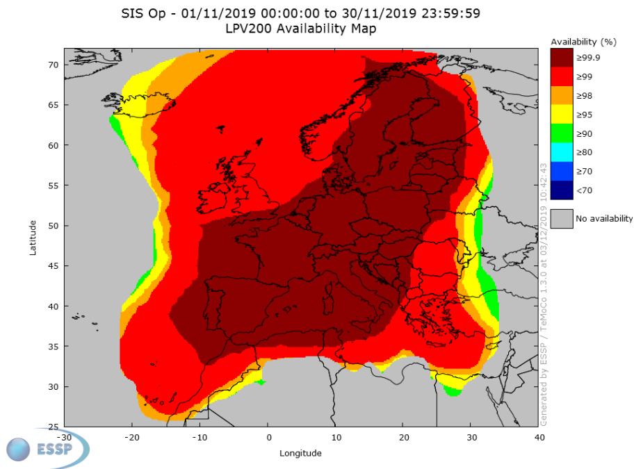
Figure 20 – EGNOS LPV-200 Availability
