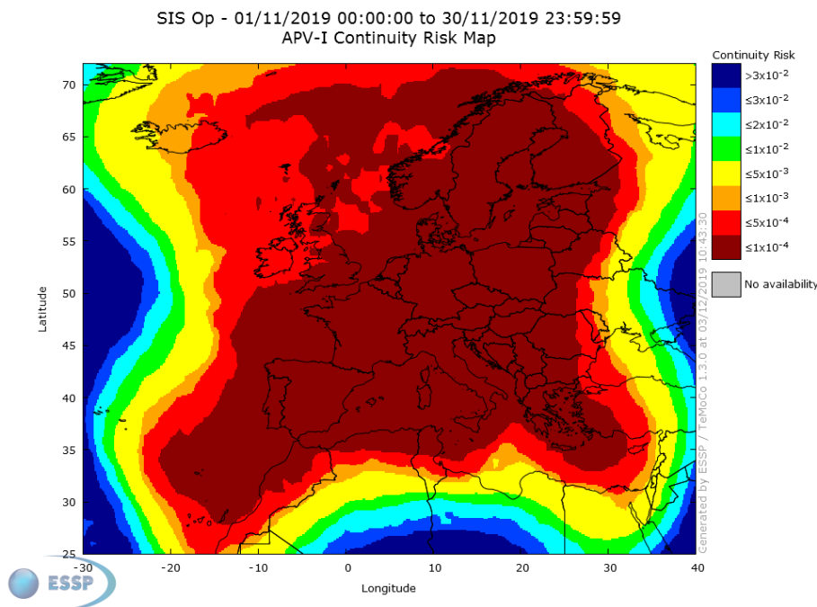
Figure 13 – EGNOS APV-I Continuity
