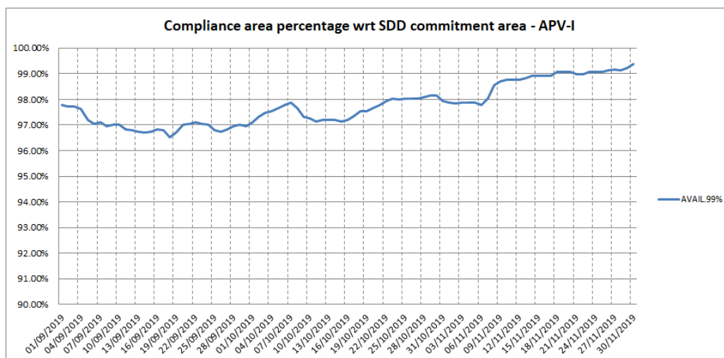
Figure 12 – EGNOS APV-I availability compliance trend
