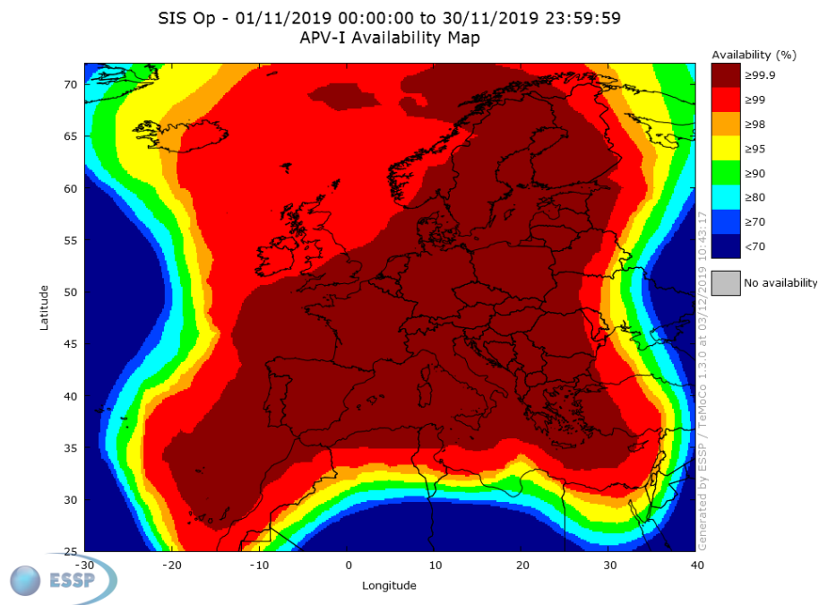
Figure 11 – EGNOS APV-I Availability
