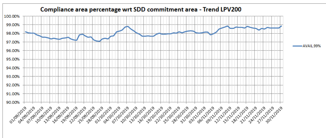
Figure 21 – EGNOS LPV-200 availability compliance trend
