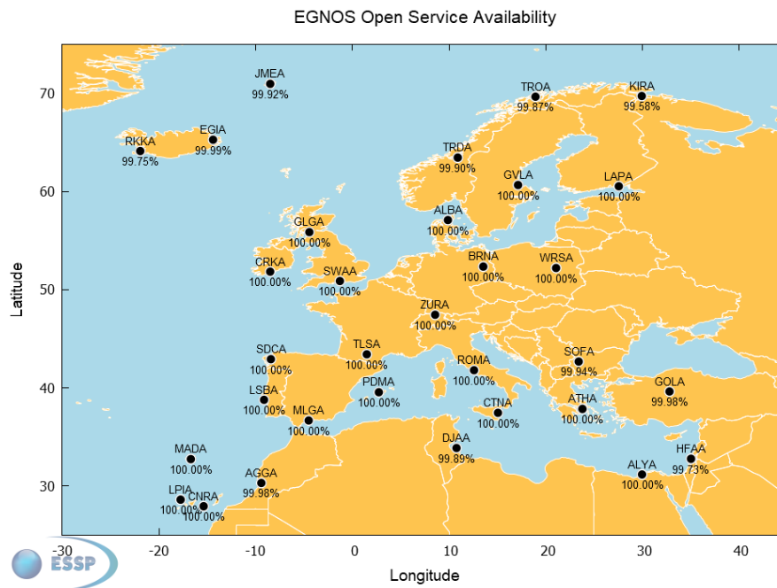
Figure 5 – EGNOS Open Service Availability at reference stations
