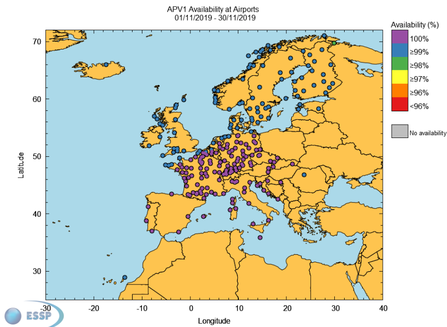
Figure 18 – EGNOS APV-I Availability at airports
