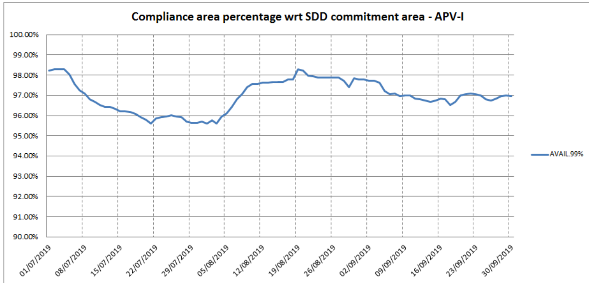
Figure 12 – EGNOS APV-I availability compliance trend
