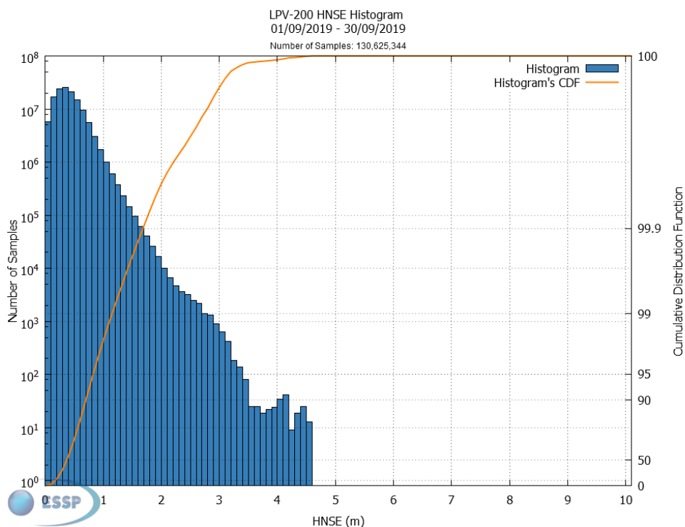
Figure 25 – EGNOS LPV-200 HNSE Histogram and Cumulative Probability
