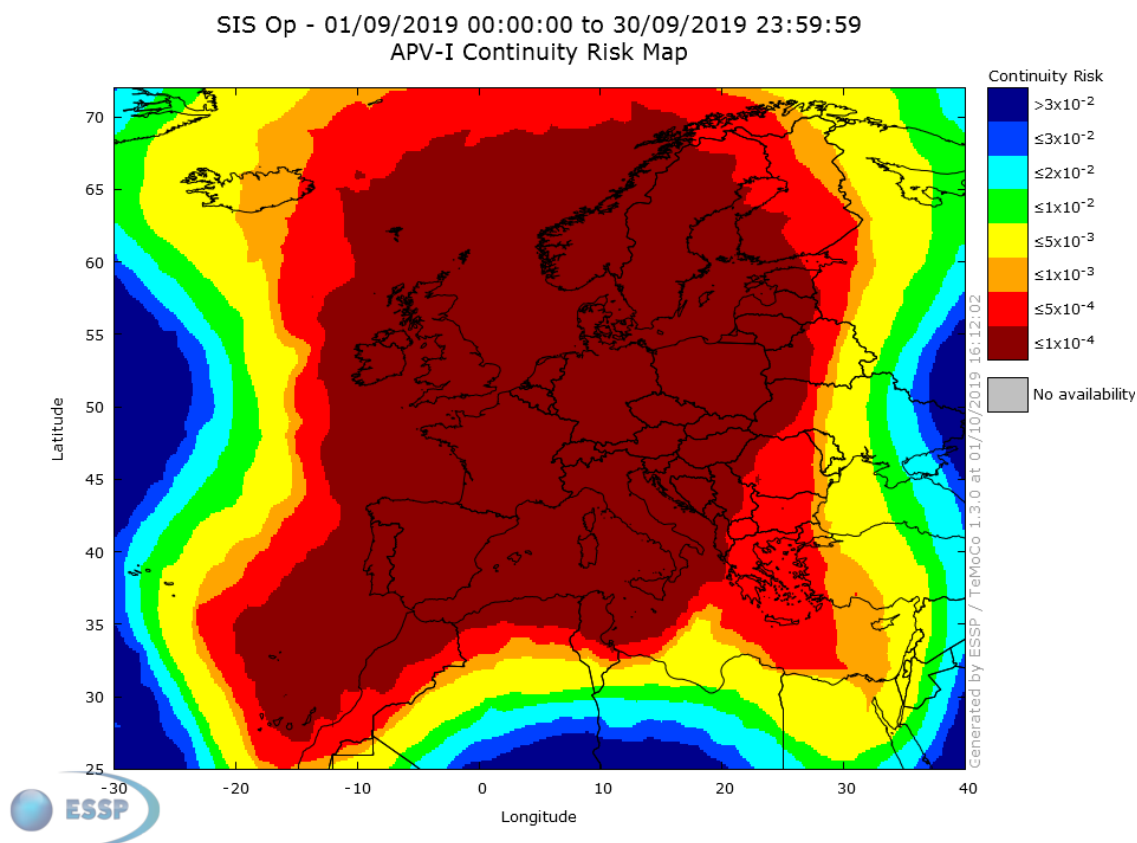
Figure 13 – EGNOS APV-I Continuity
