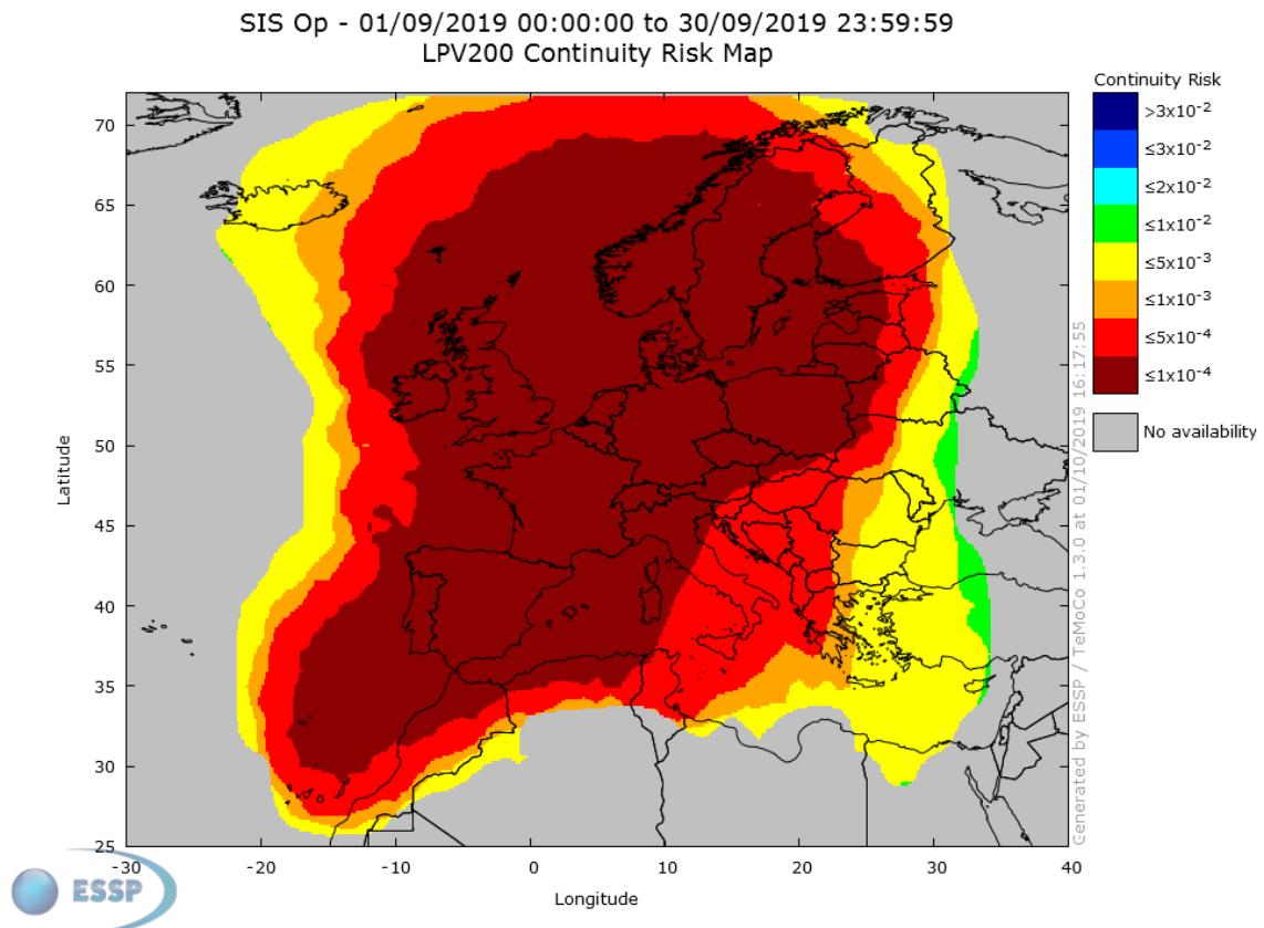
Figure 22 – EGNOS LPV-200 Continuity 2
