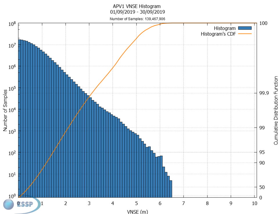
Figure 17 – EGNOS APV-I VNSE Histogram and Cumulative Probability
