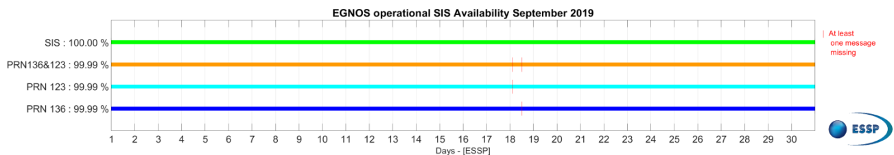
Figure 1 – EGNOS SIS & PRN Availability for September 2019.
