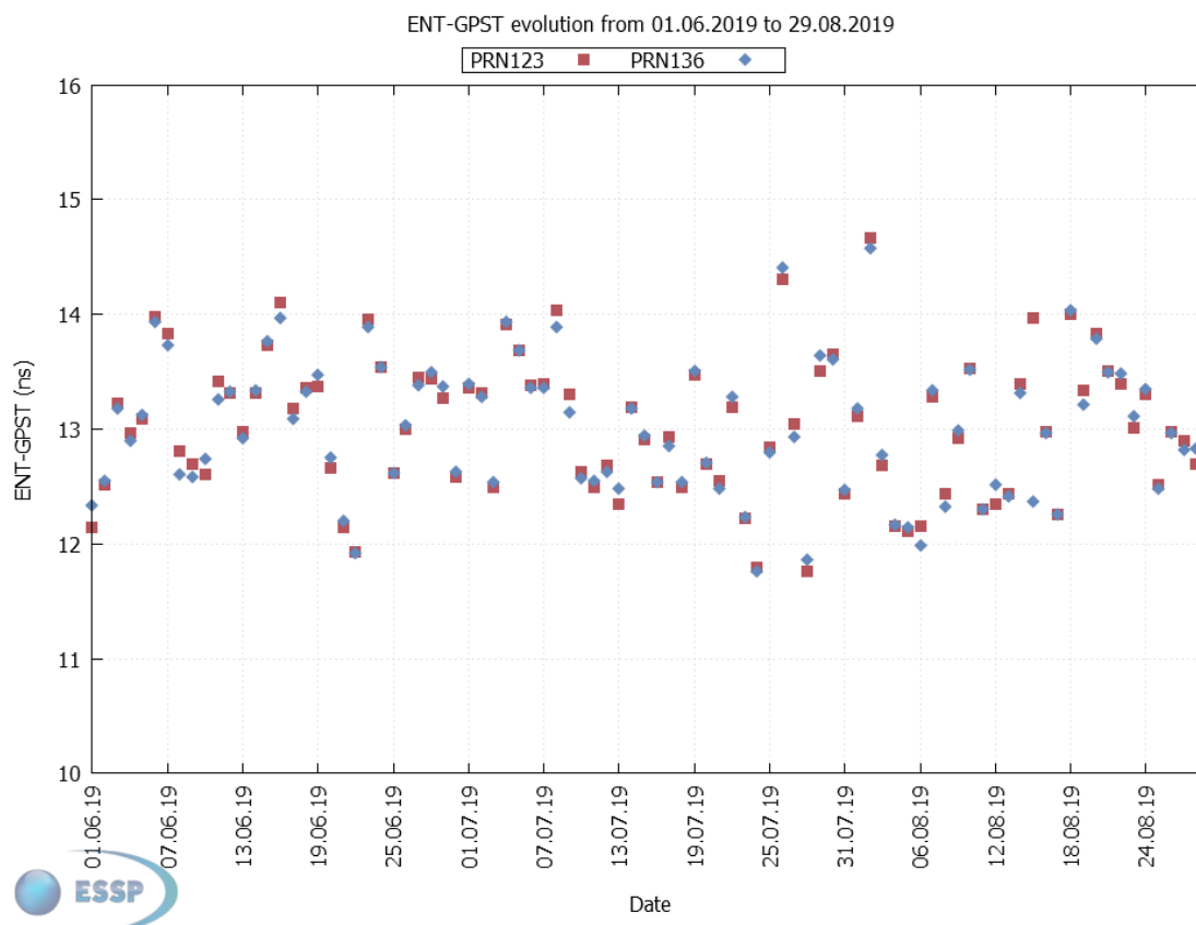
Figure 30 – ENT-GPS offset evolution
