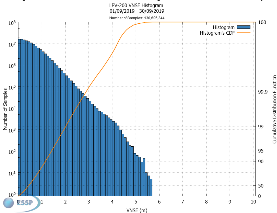
Figure 26 – EGNOS LPV-200 VNSE Histogram and Cumulative Probability
