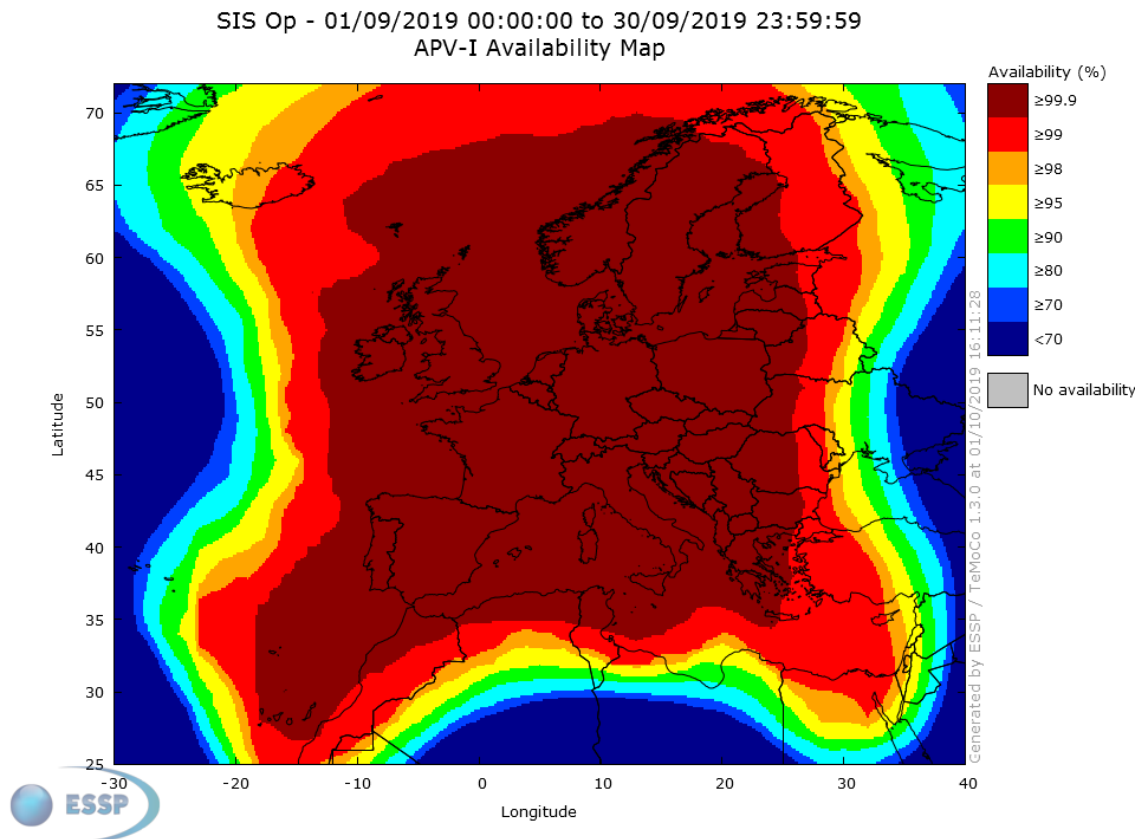
Figure 11 – EGNOS APV-I Availability
