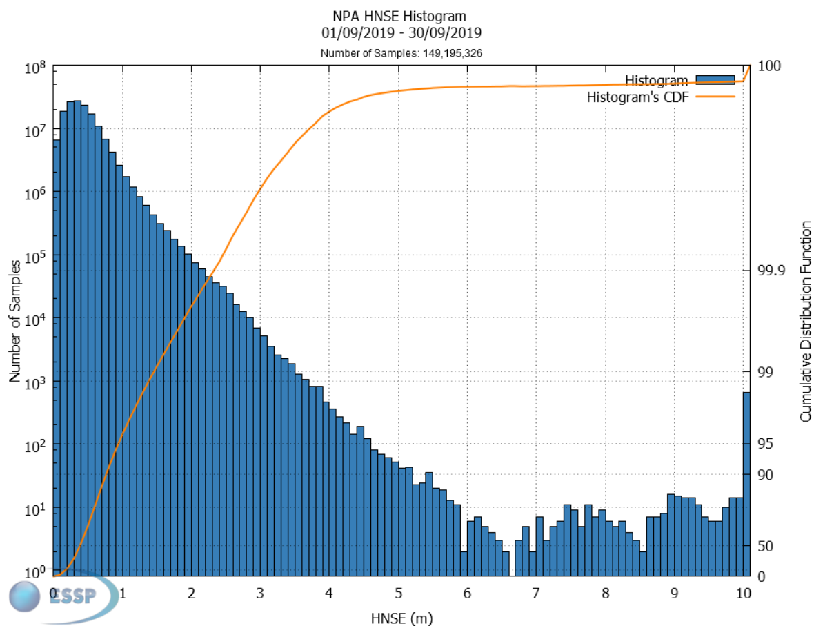
Figure 10 – EGNOS NPA HNSE Histogram and Cumulative Probability
