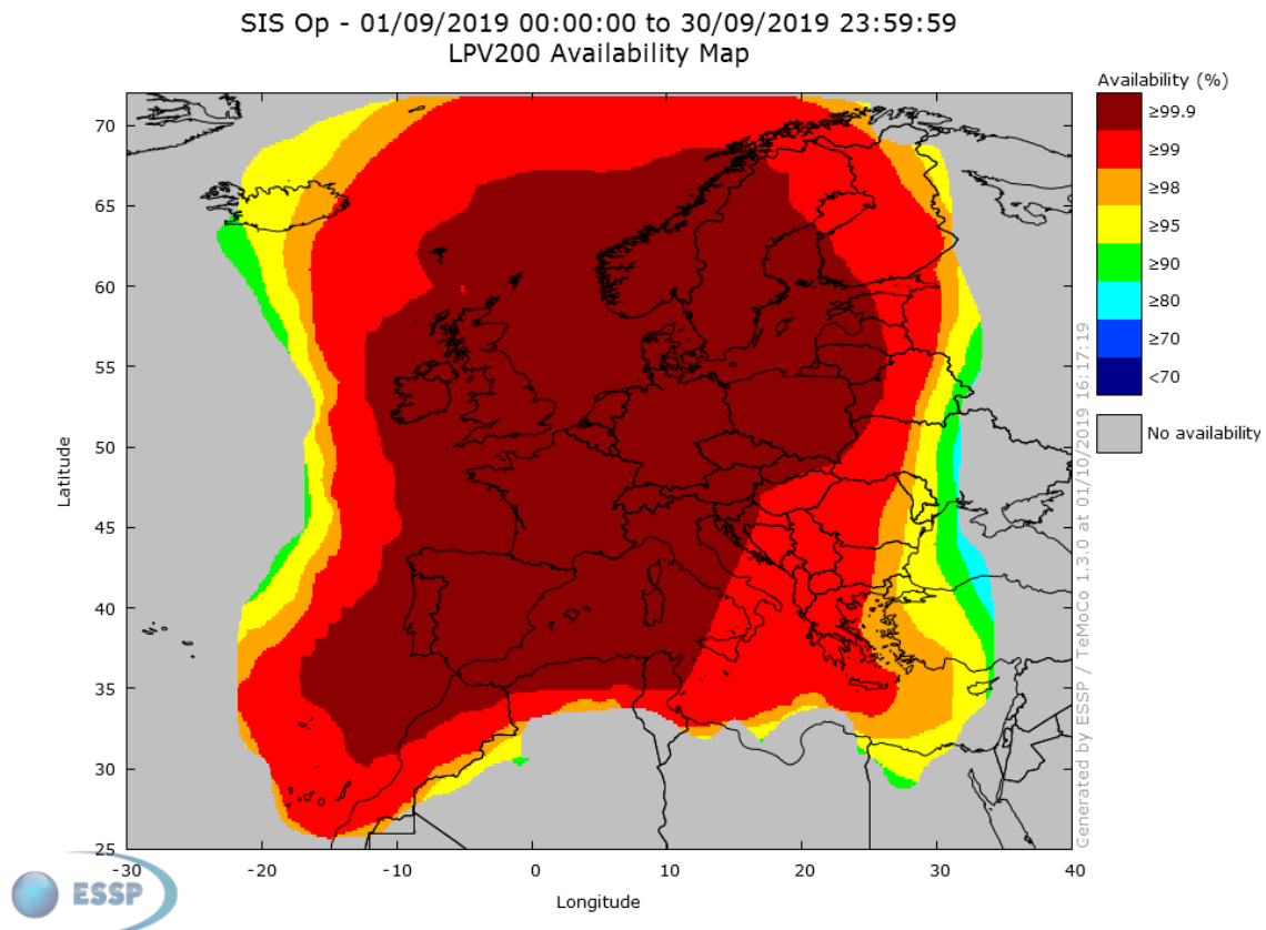
Figure 20 – EGNOS LPV-200 Availability
