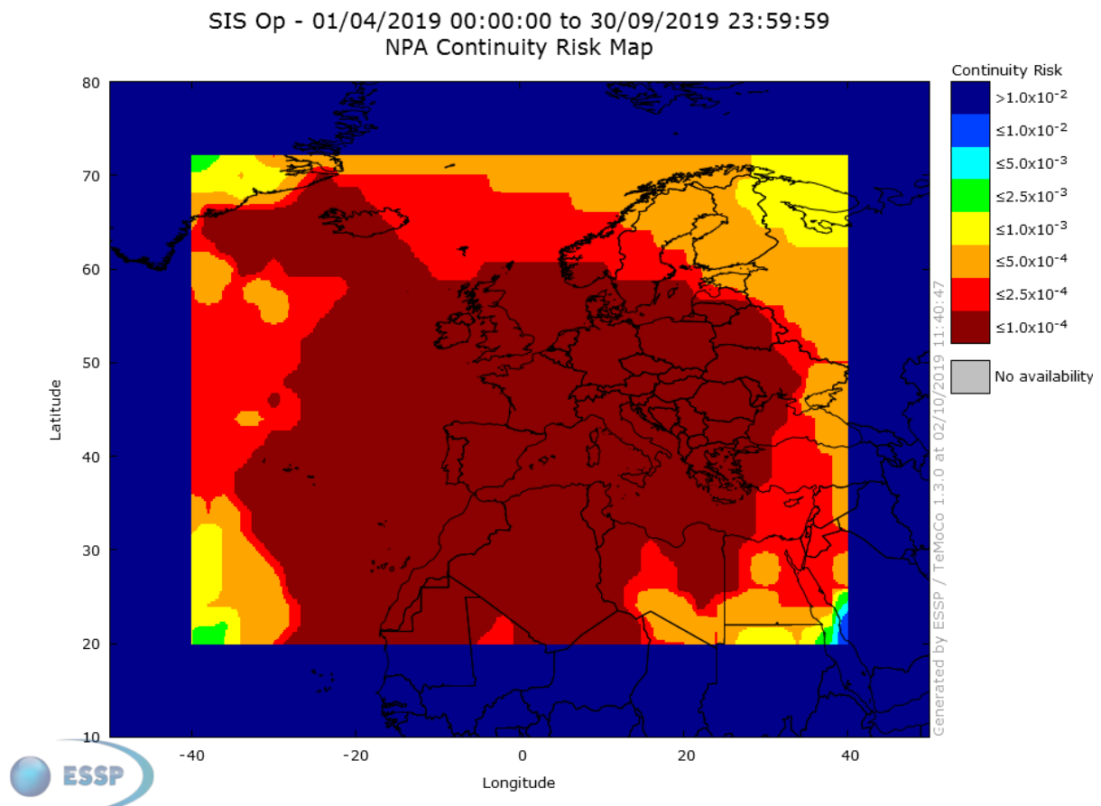
Figure 8 – EGNOS NPA Continuity over the last 6 months
