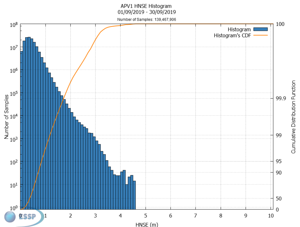
Figure 16 – EGNOS APV-I HNSE Histogram and Cumulative Probability
