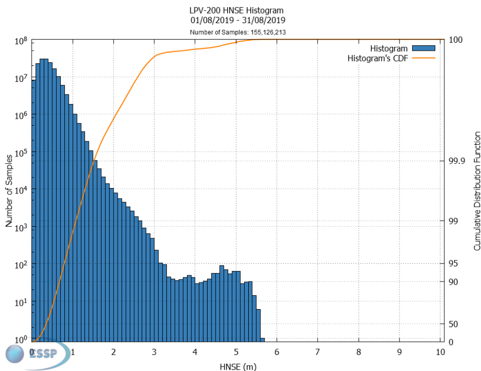
Figure 25 – EGNOS LPV-200 HNSE Histogram and Cumulative Probability
