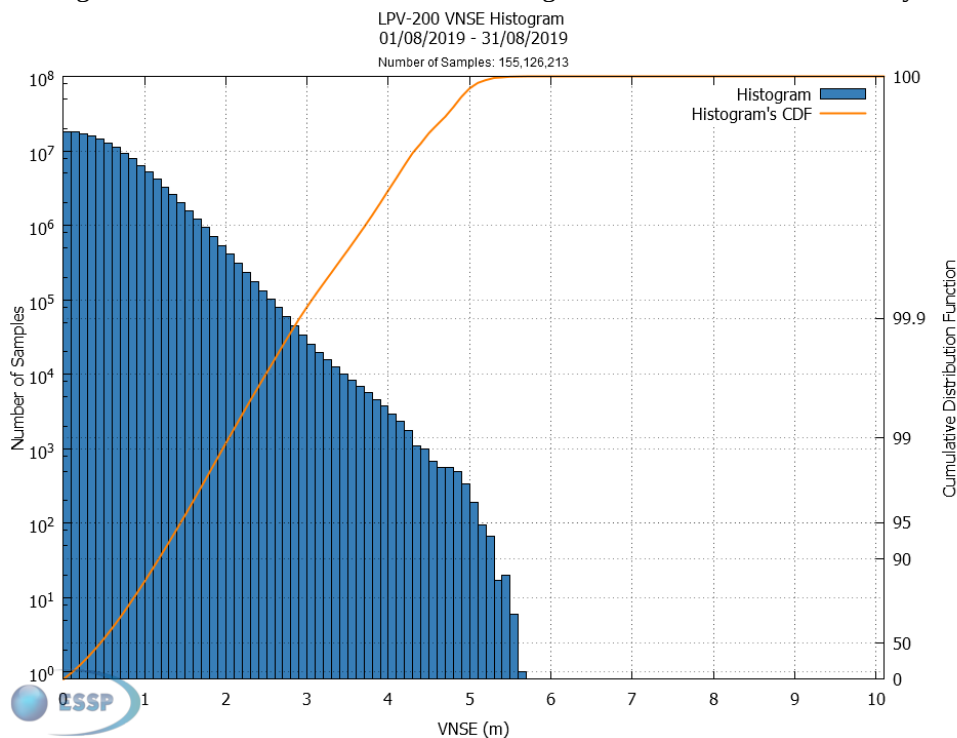
Figure 26 – EGNOS LPV-200 VNSE Histogram and Cumulative Probability
