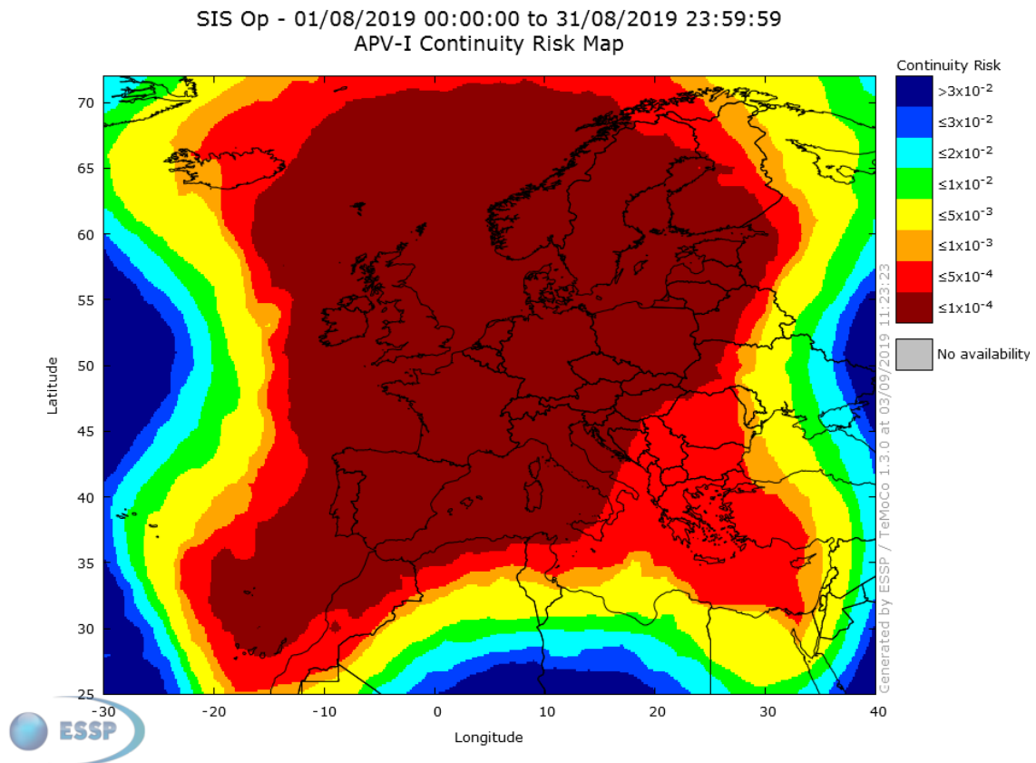
Figure 13 – EGNOS APV-I Continuity
