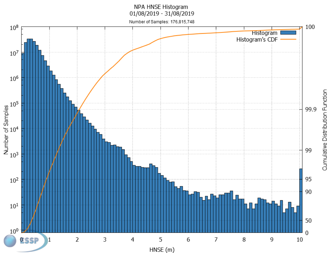
Figure 10 – EGNOS NPA HNSE Histogram and Cumulative Probability
