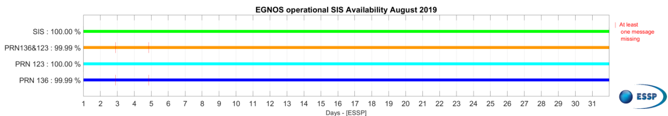
Figure 1 – EGNOS SIS & PRN Availability for August 2019.
